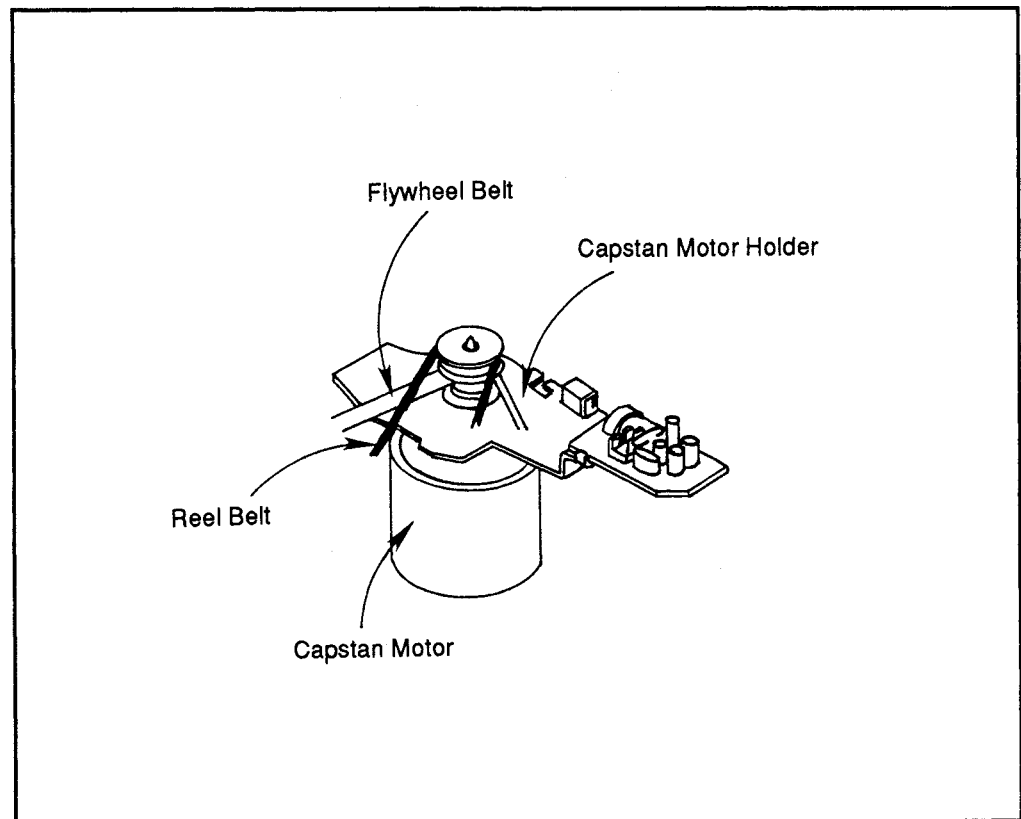
Figure 39: Capstan motor assembly
