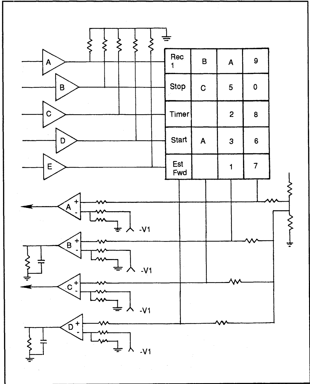
Figure 2: Interrupt connections to keyboard
