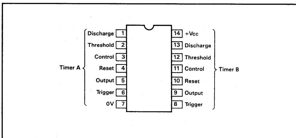
Figure 3: 556 dual-timer pin connections
