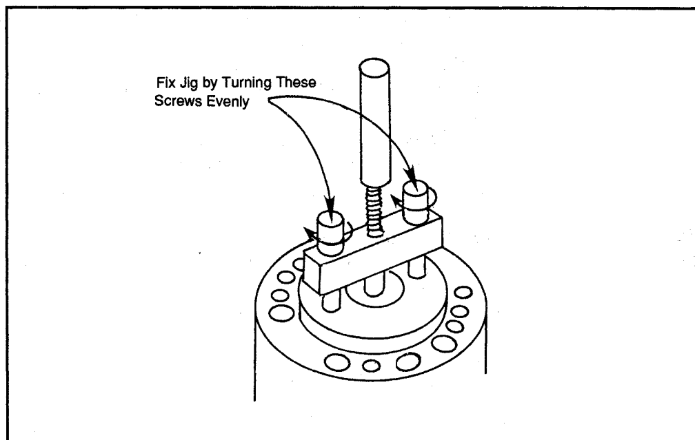
Figure 8: Extracting jig
