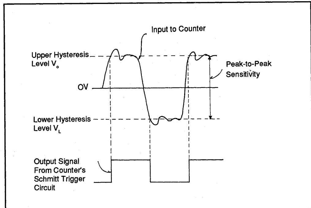
Figure 3: Schmitt trigger
