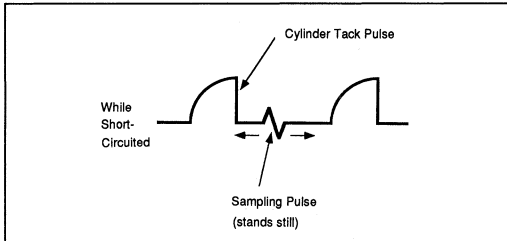
Figure 19: Cylinder tach pulse and sampling pulse
