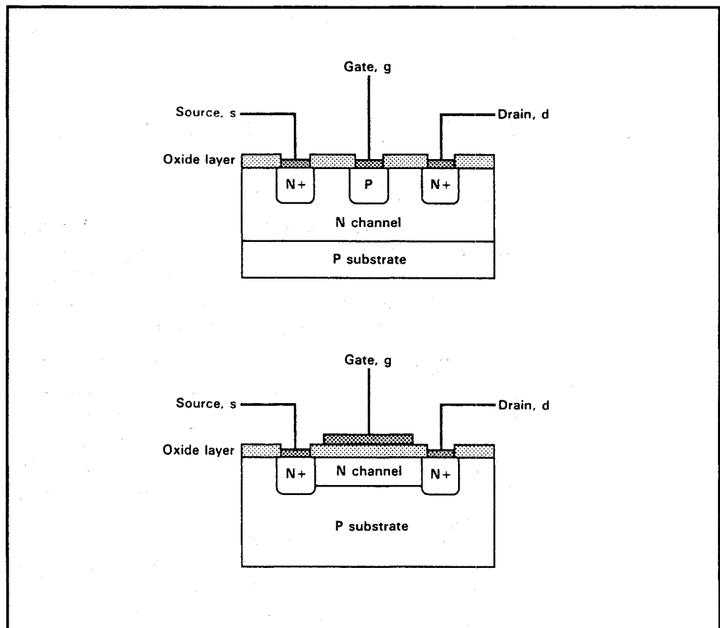
Figure 6: JFET (top) and IGFET (bottom) FETs
