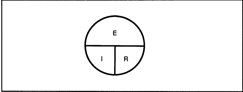
Figure 1: Ohm's Circle
