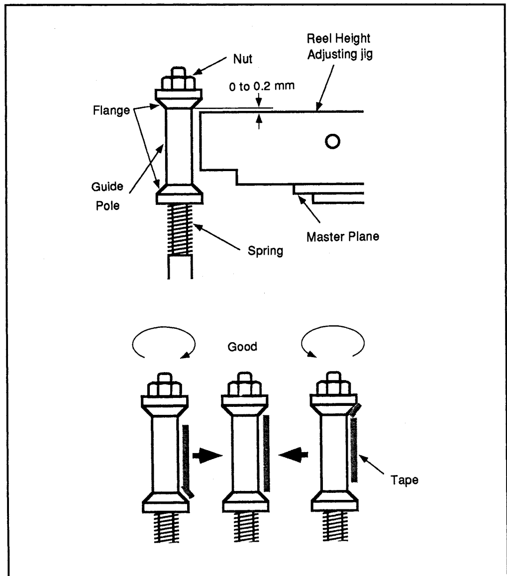
Figure 12: Guide post height adjustment
