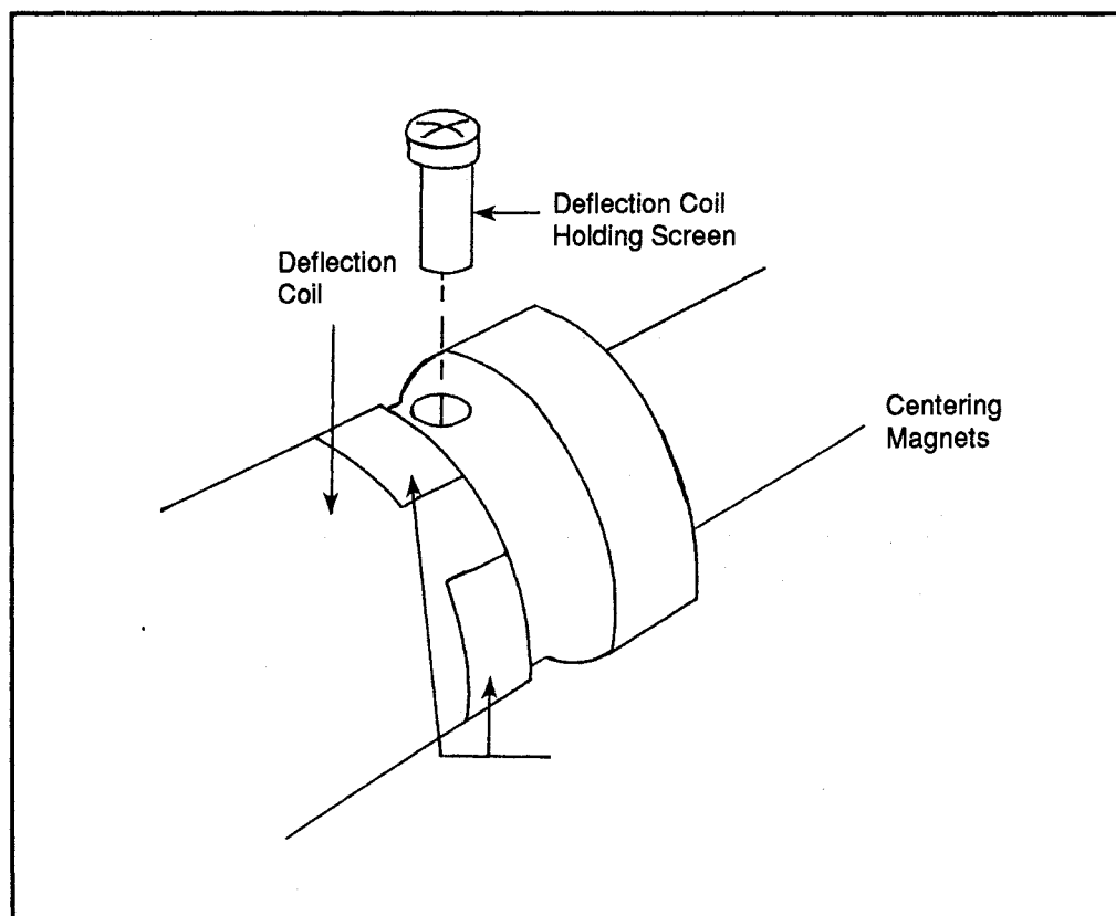
Figure 5: Deflection coil holding screw
