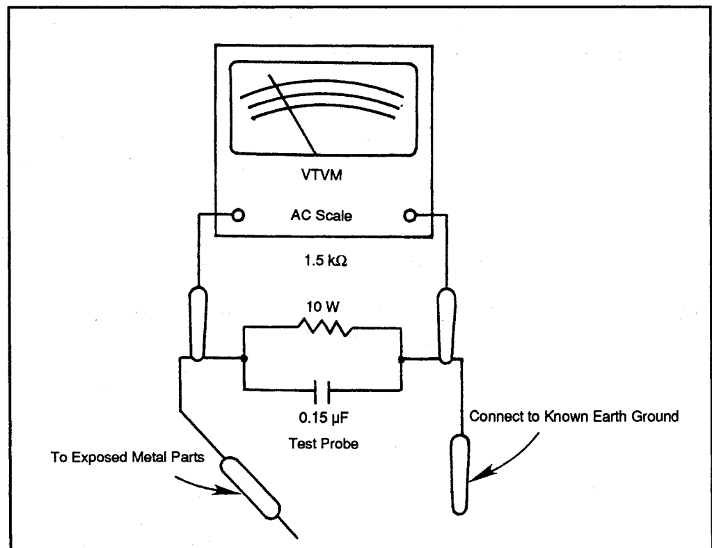
Figure 2: Arrangement to test for possible current leakage
