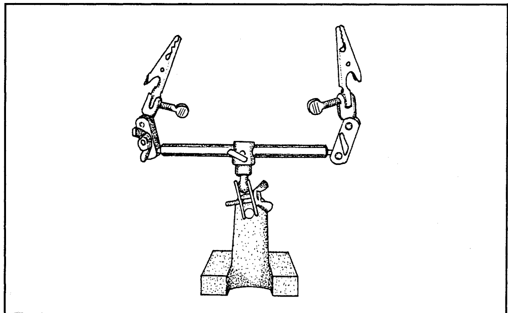
Figure 4: "Helping hand"
