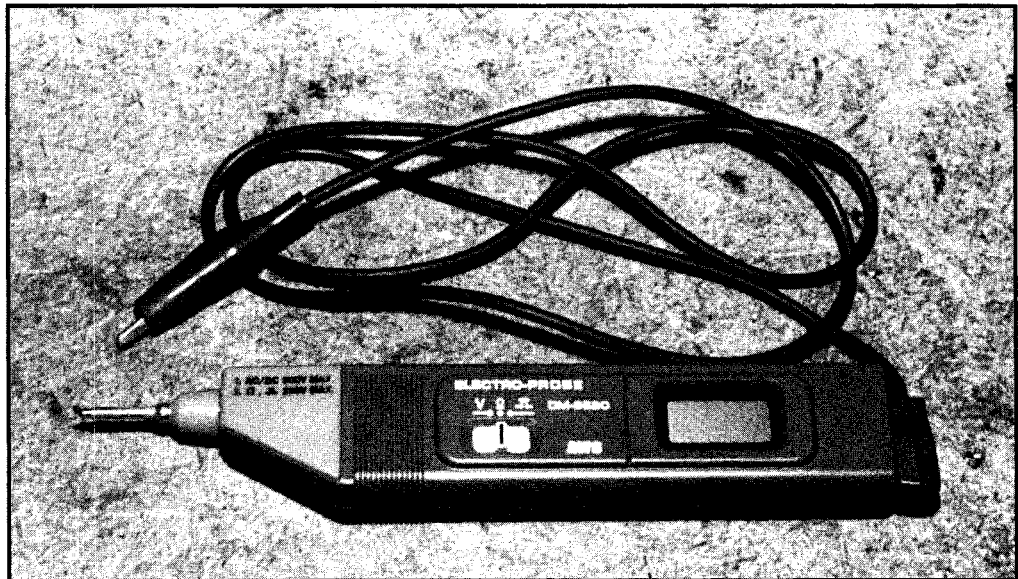
Figure 3: Logic pulsar
