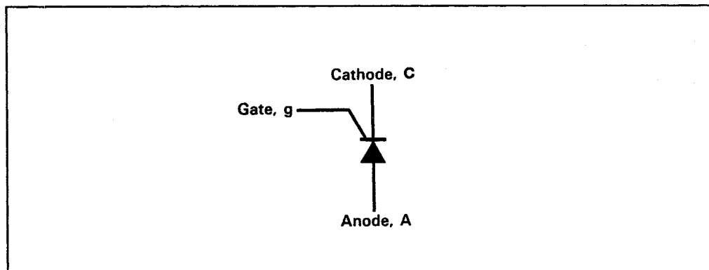
Figure 1: Thyristor symbol and terminal connections
