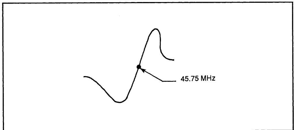
Figure 6: AFT waveform used for adjustments
