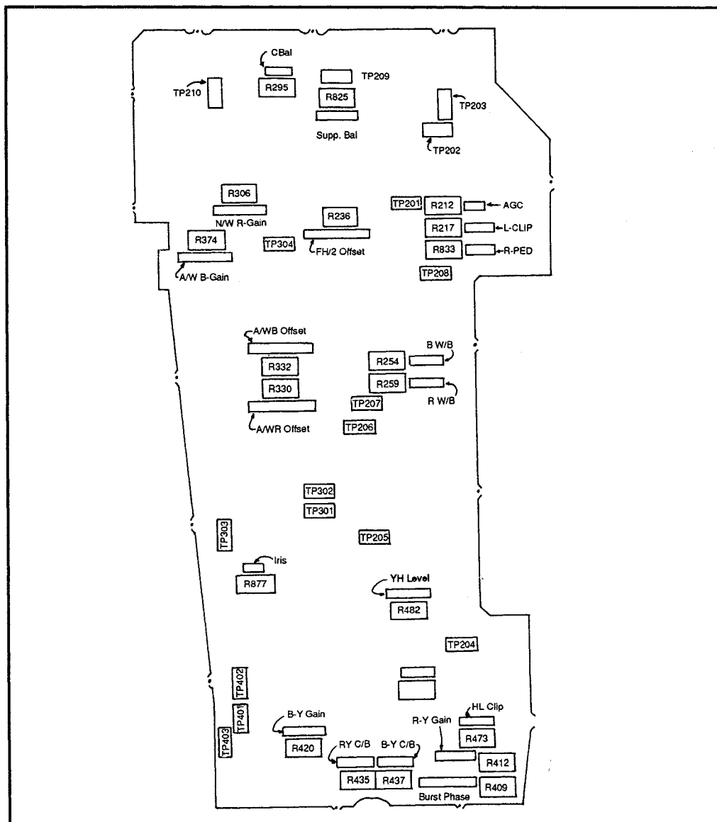
Figure 12: Location of test points and controls on encorder board
