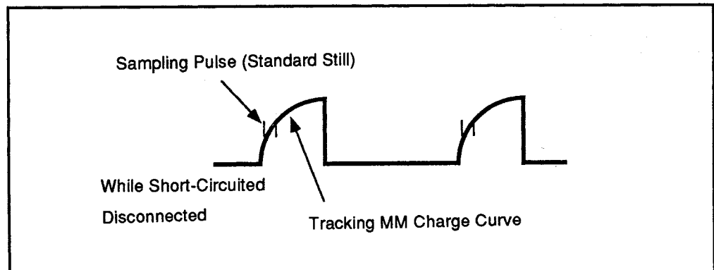
Figure 22: Capstan waveform adjustment without circuit shorted
