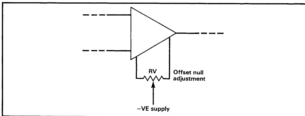
Figure 3: Offset-null facility
