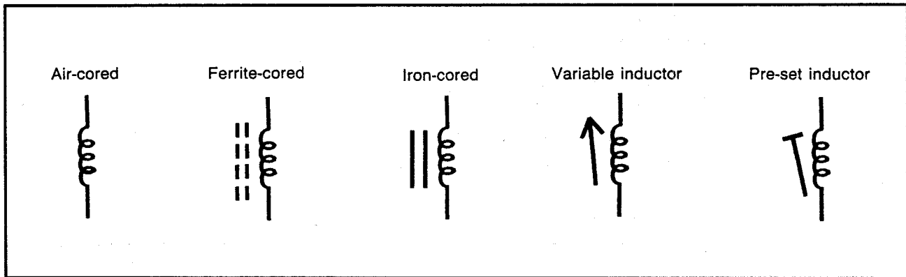
Figure 1: Inductor symbols
