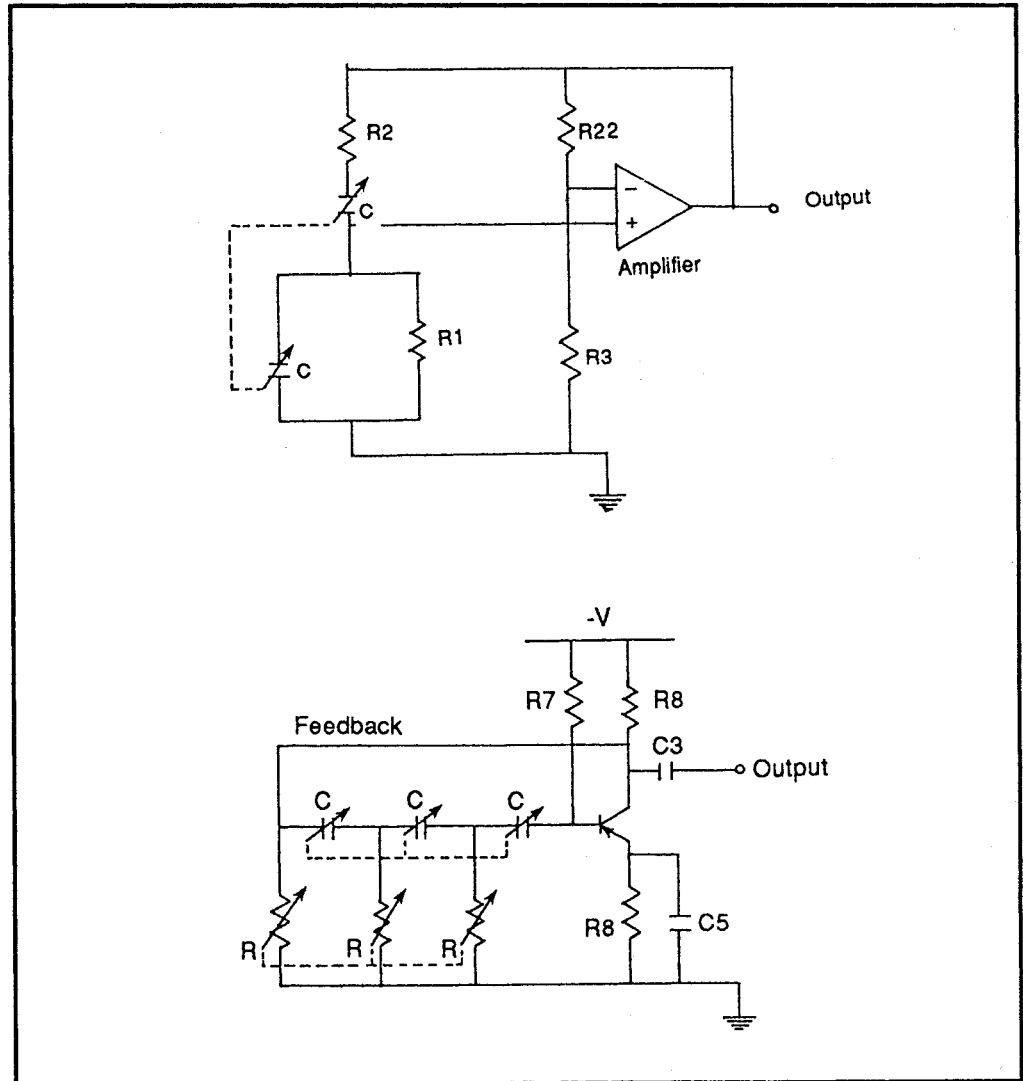
Figure 2: Oscillator circuit
