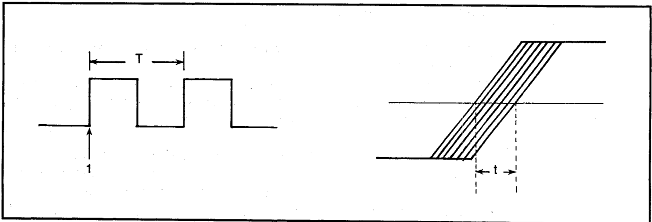
Figure 9: Waveform jitter measurement: (a) square wave (b) display of intensified part of waveform using the delay time base.
