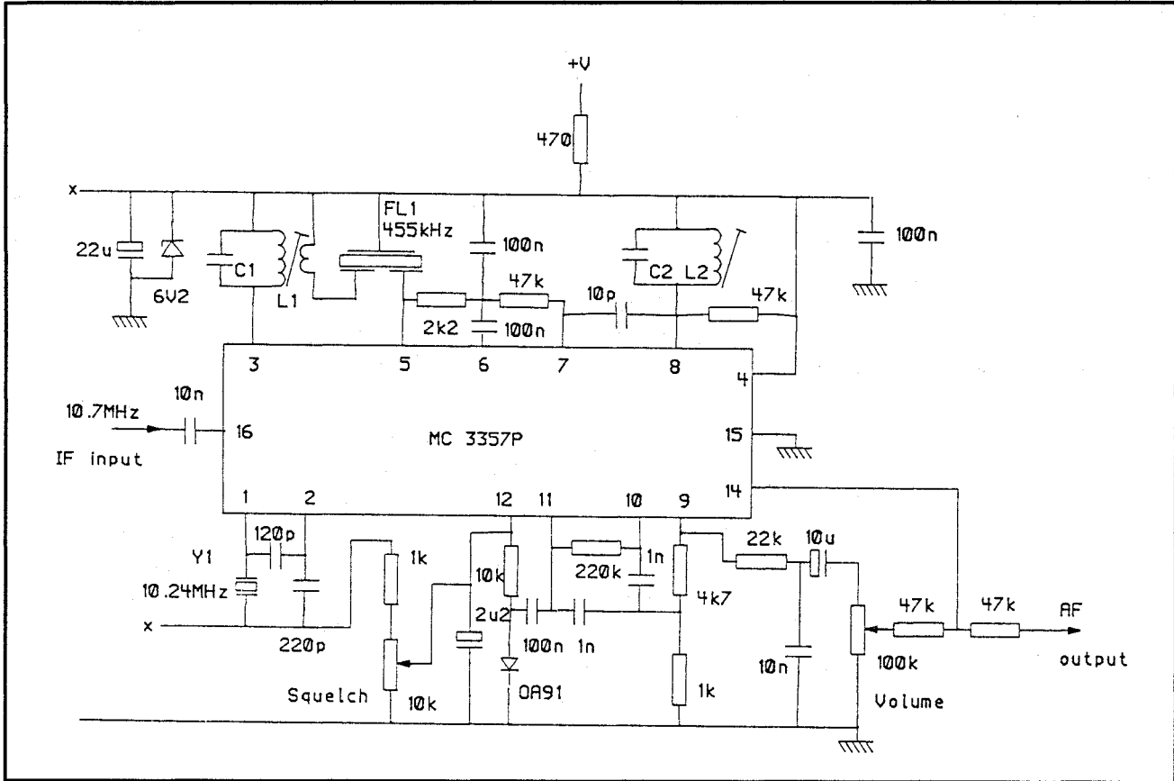
Figure 3: IC based IF amplifier circuit
