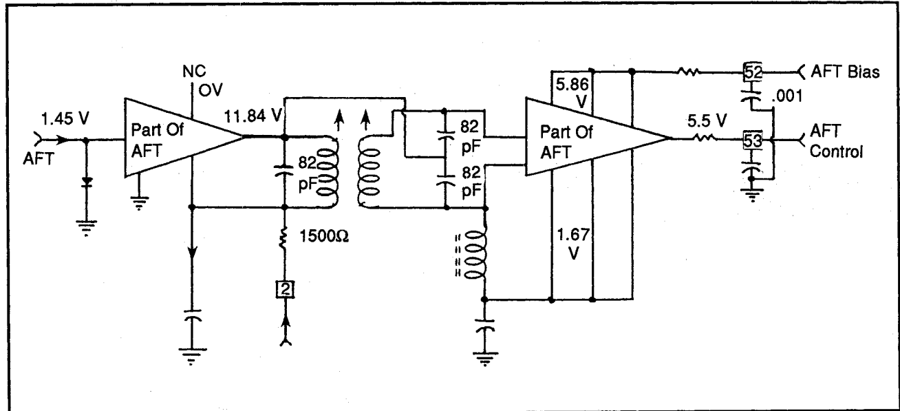
Figure 13: AFT circuit diagram
