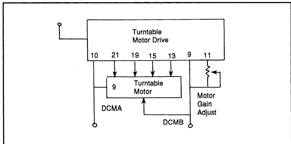
Figure 1: Disc motor adjustment
