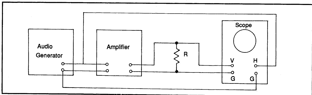
Figure 16: A typical audio generator hookup
