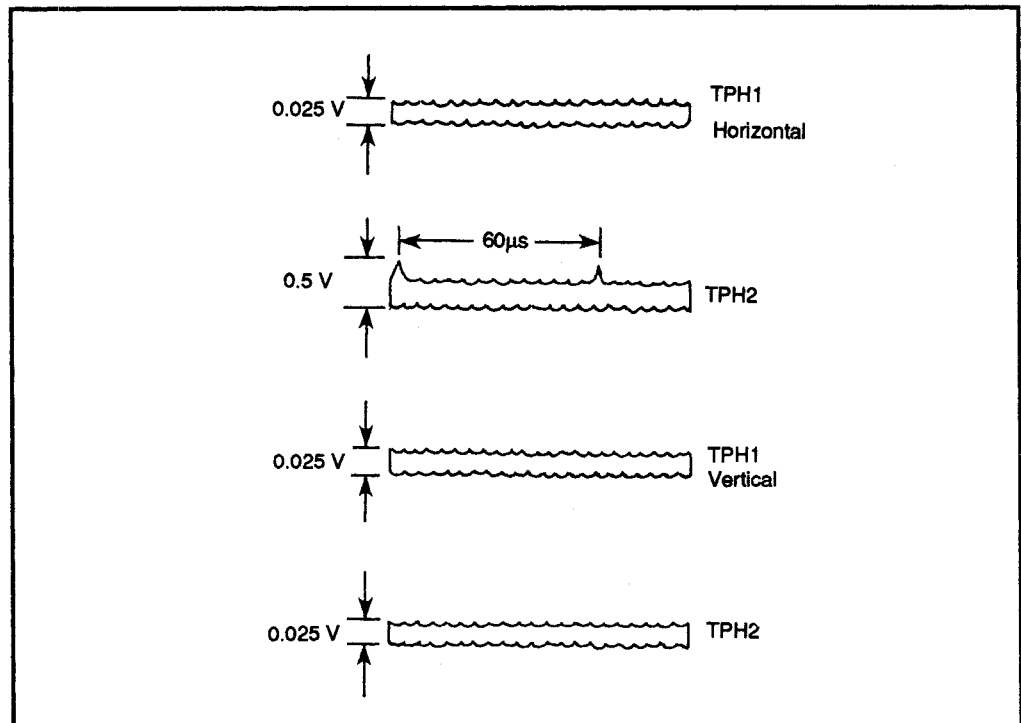
Figure 1: R and B signal shading release waveforms
