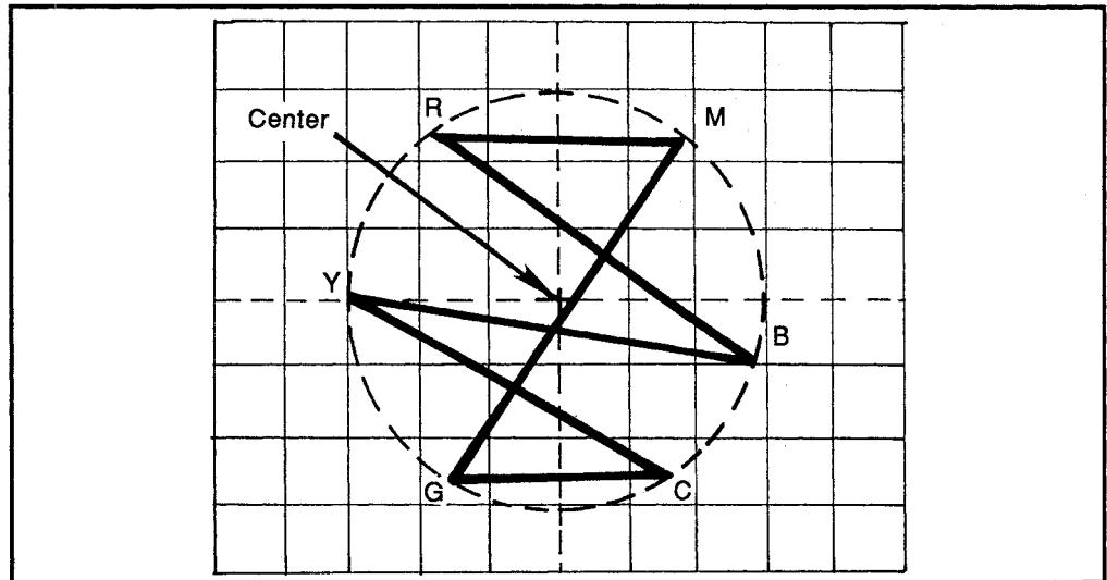
Figure 9: Baseline curvature
