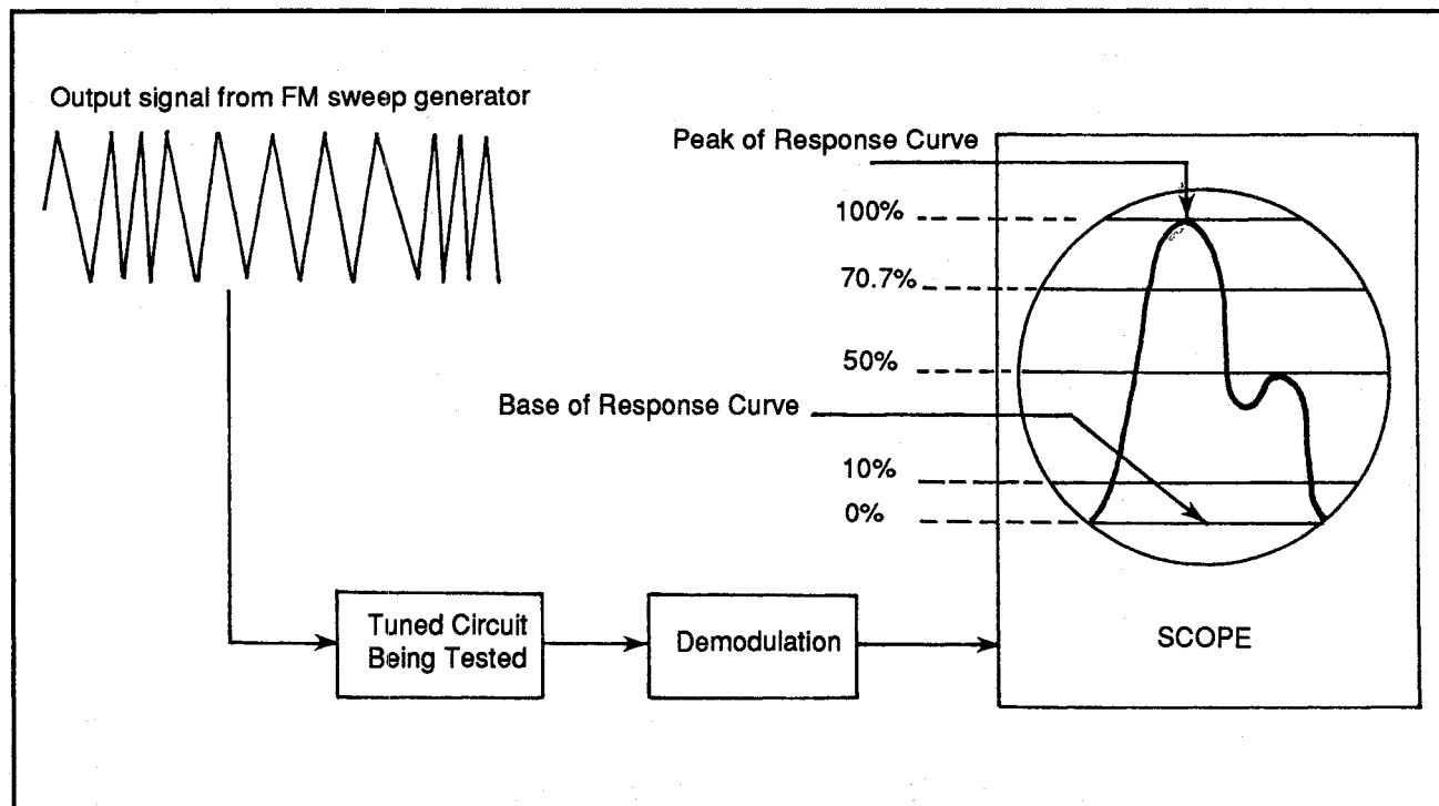
Figure 13: Basic principle of sweep alignment
