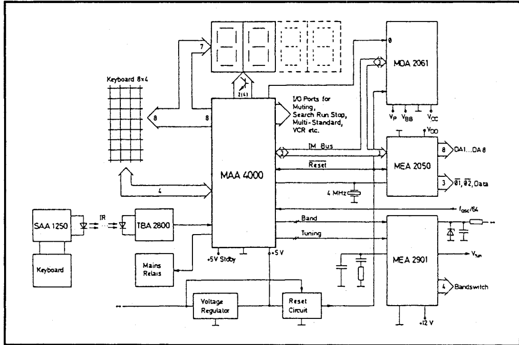
Figure 5: IC tuner circuit
