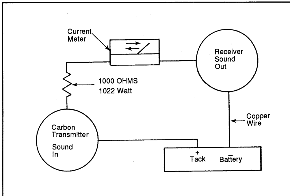
Figure 6: Simple, but operational telephone
