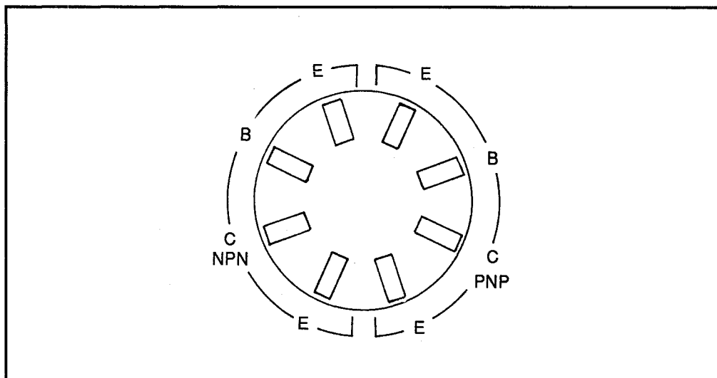
Figure 11: Test socket configuration
