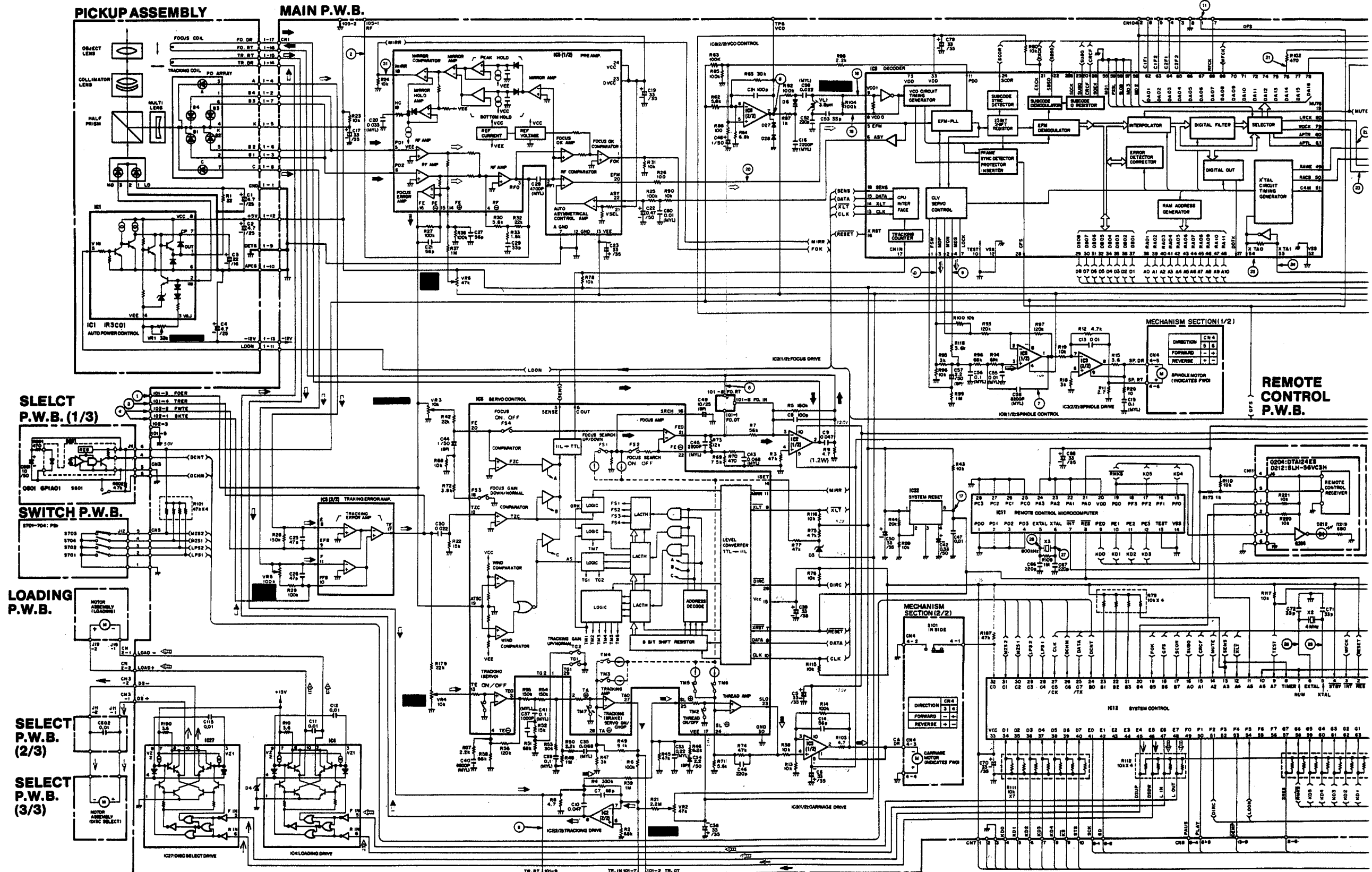
DA-C60 circuit diagram
