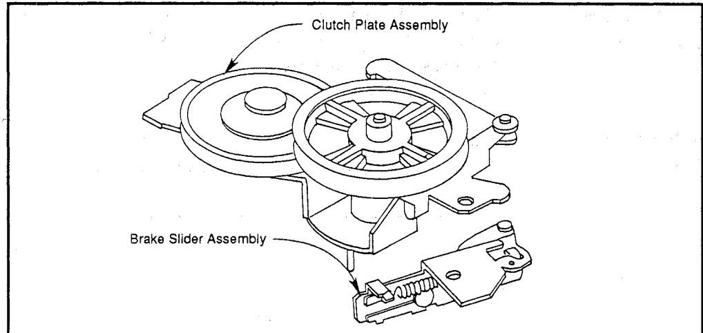
Figure 41: Clutch plate assembly
