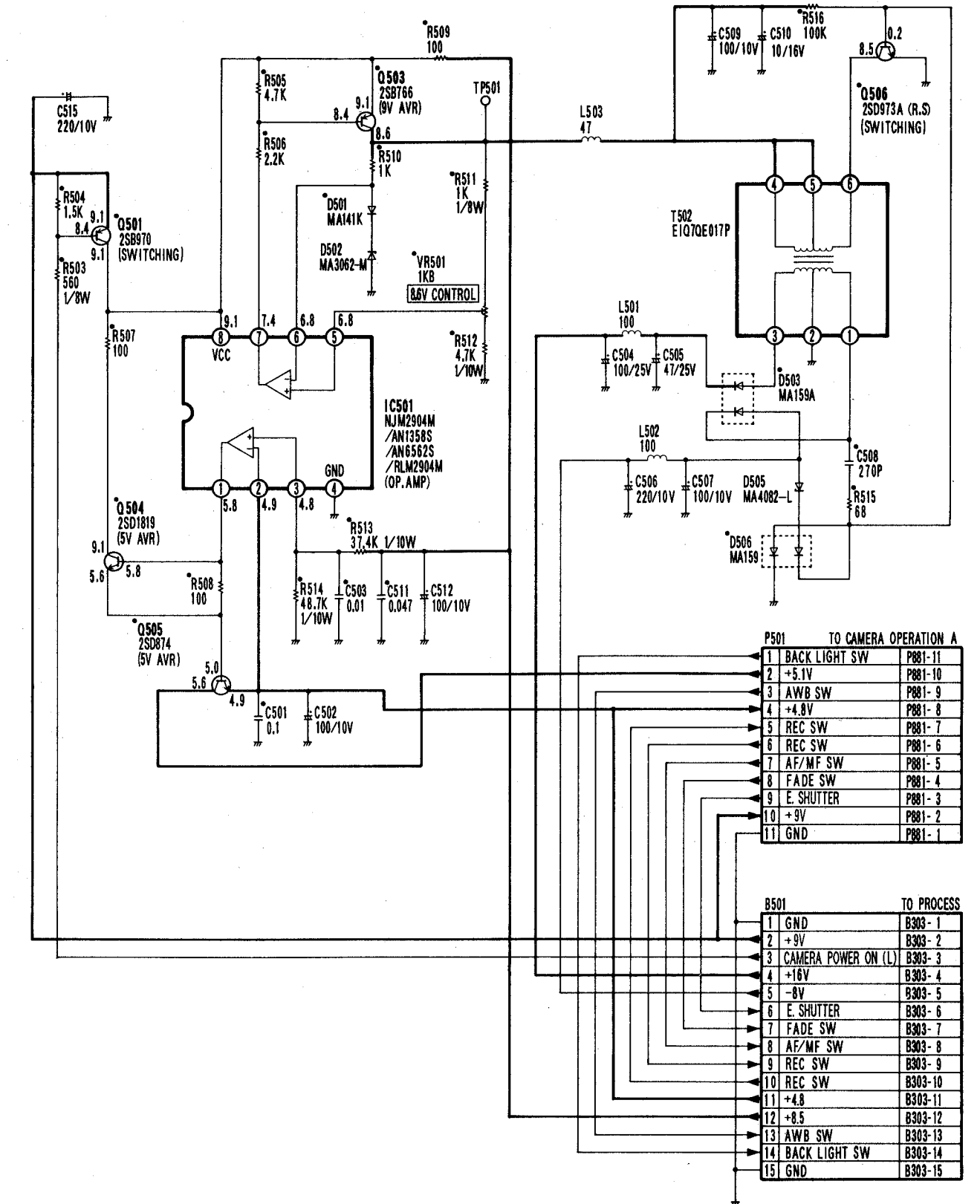
PV-602, PV-604 and PV-610 camera power supply schematic
