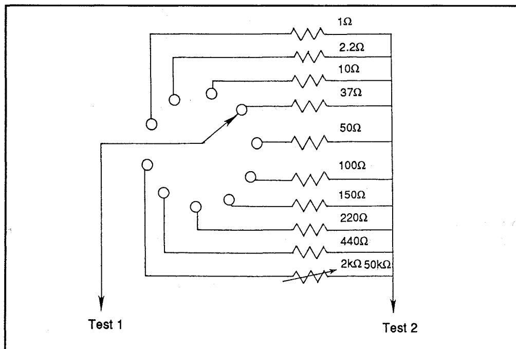
Figure 8: Resistance substitution circuit
