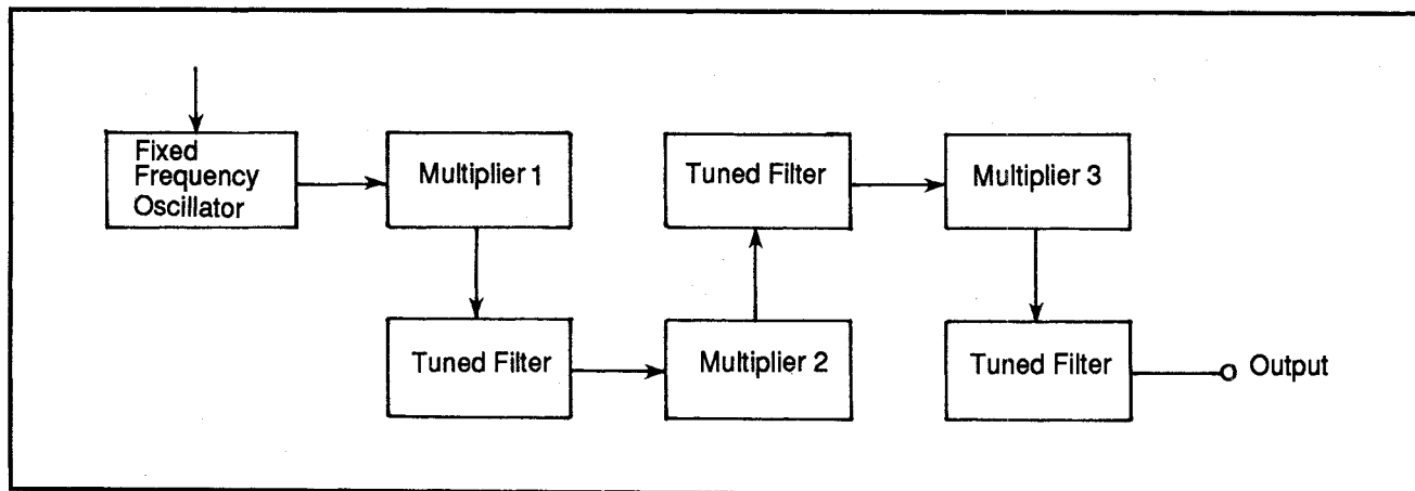
Figure 9: Frequency multiplier
