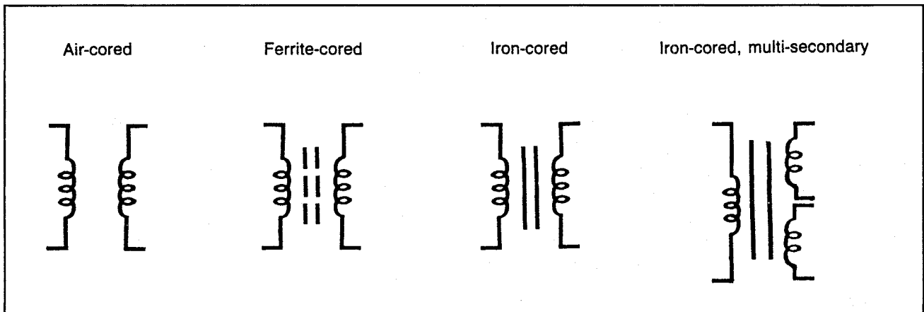
Figure 1: Transformer symbols
