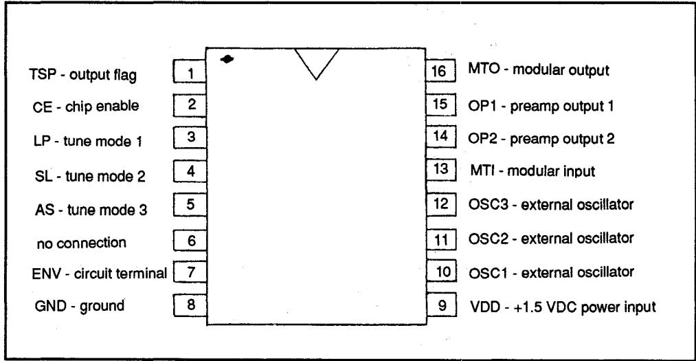
Figure 3: Logic on the UM3482A doorbell music chip
