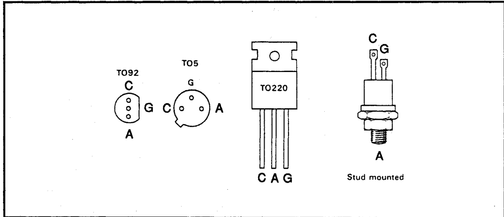
Figure 2: Thyristor casings
