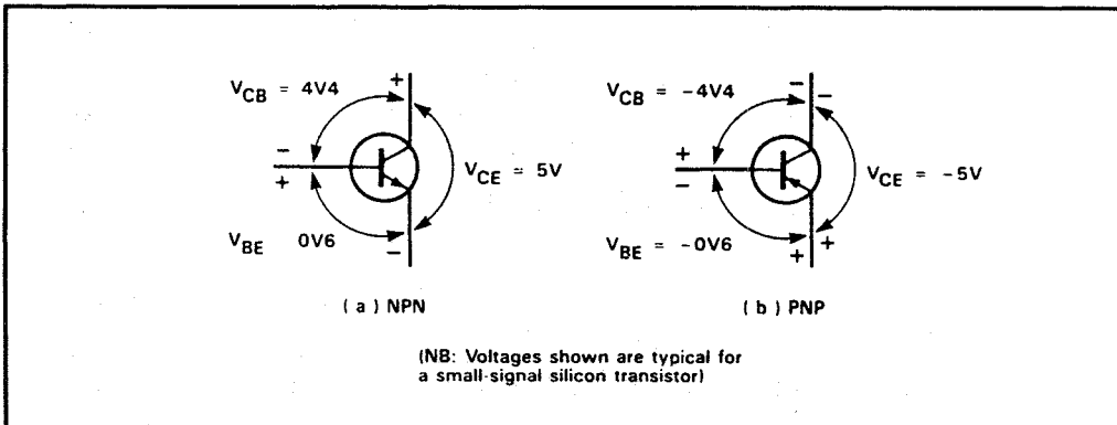
Figure 5: Bipolar transistors potentials, biased for linear operation
