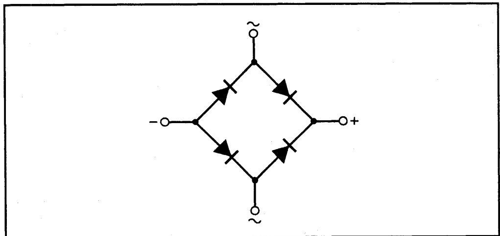
Figure 4: Bridge rectifier
