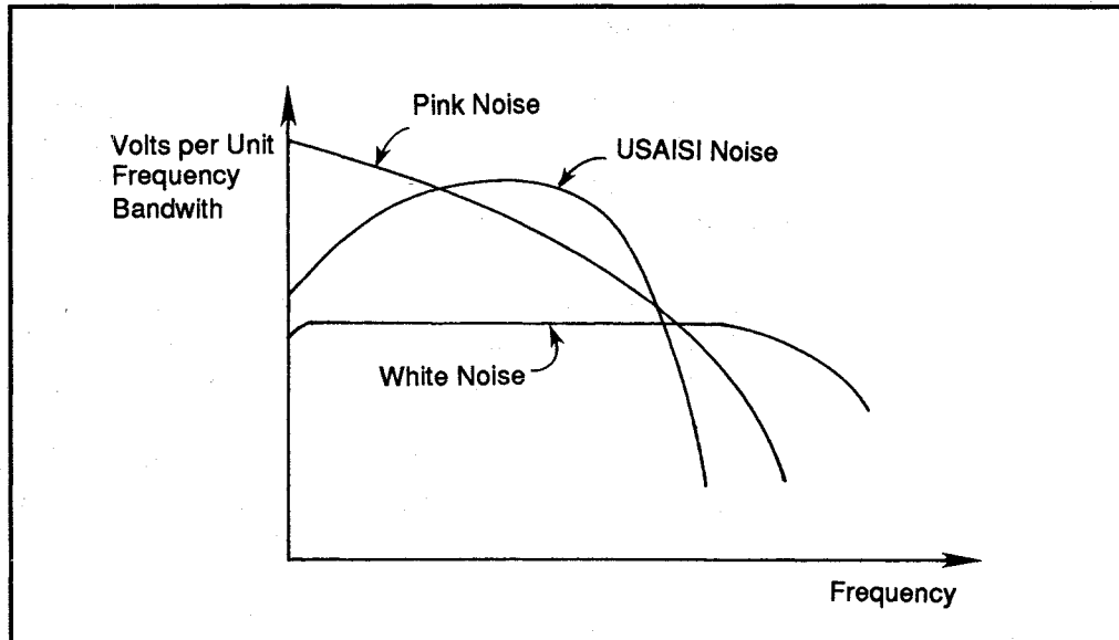
Figure 13: Three possible curves of the noise-power spectrum
