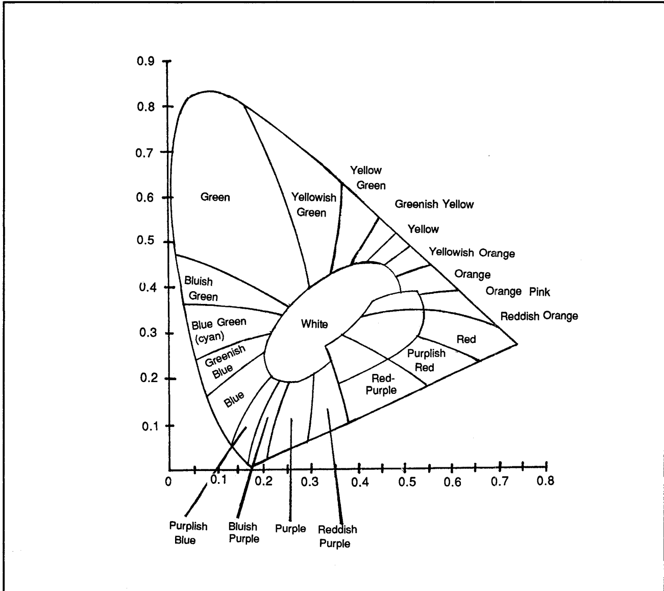
Figure 1: Chromaticity diagram
