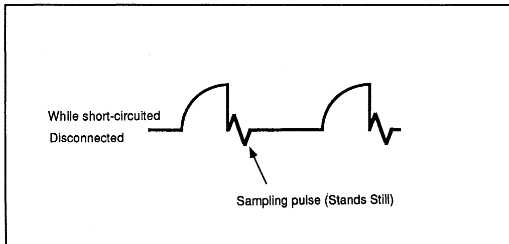
Figure 20: Cylinder tach pulse and sampling pulse after short circuit removed
