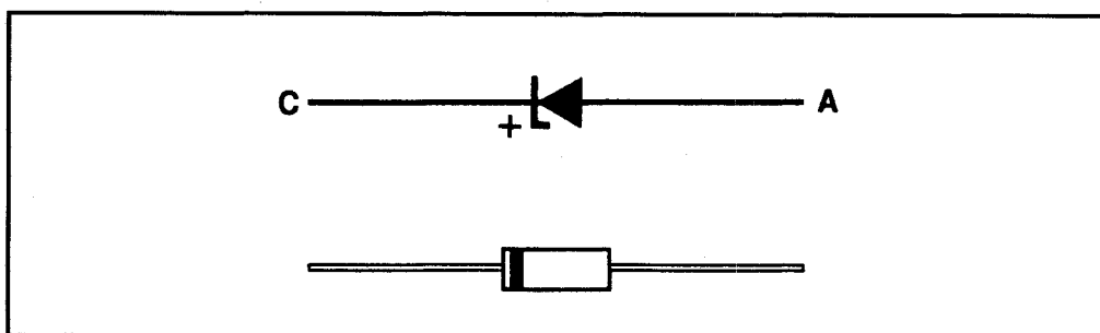
Figure 6: Zener diode symbol and typical casing
