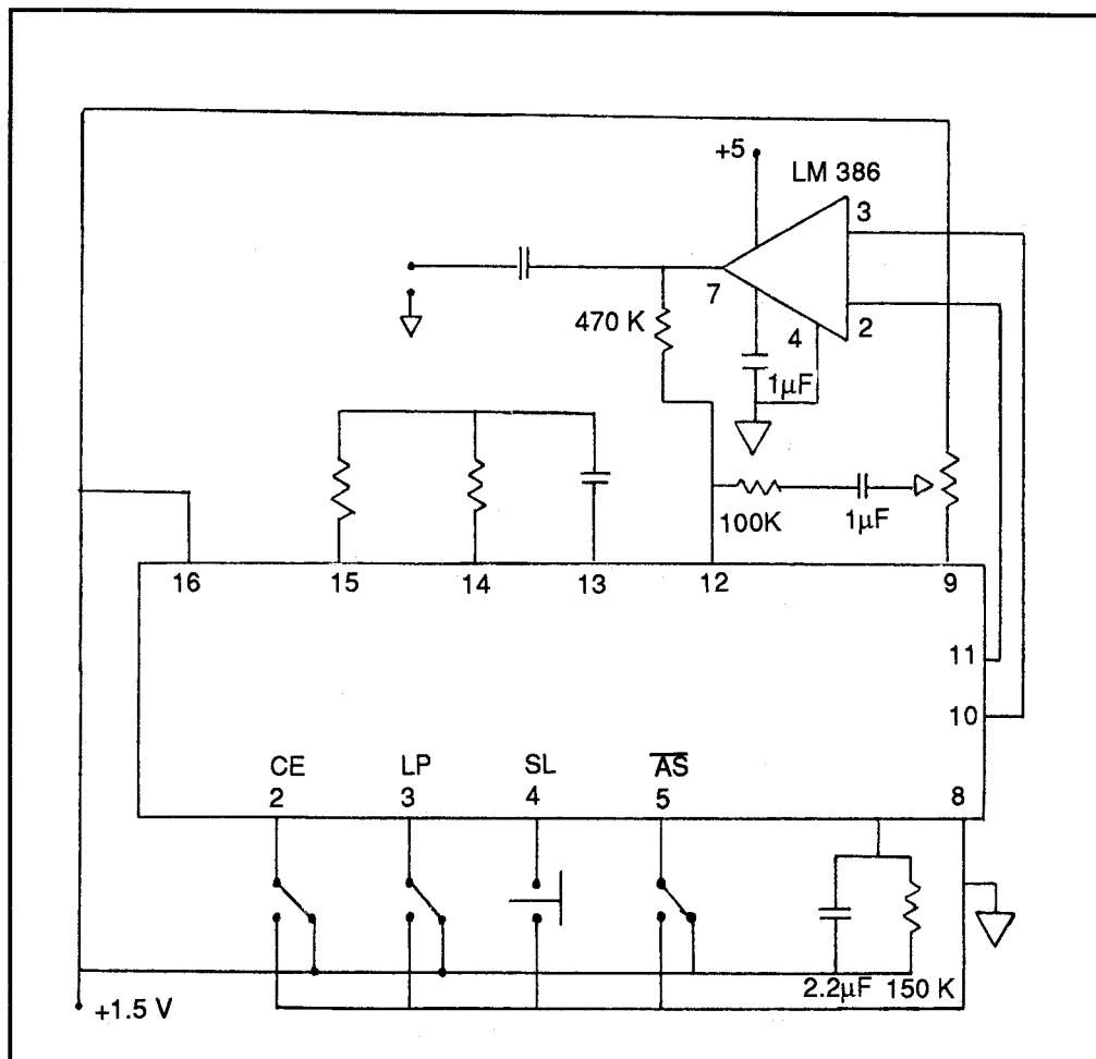
Figure 2: Melody doorbell using the UMA3482A chip
