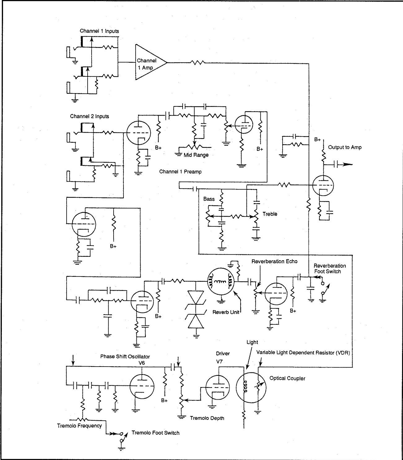
Figure 1: Tube-type preamplifier
