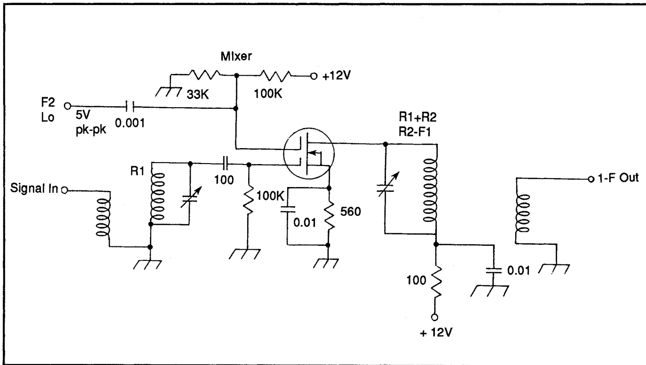
Figure 3: Mixer stage circuit
