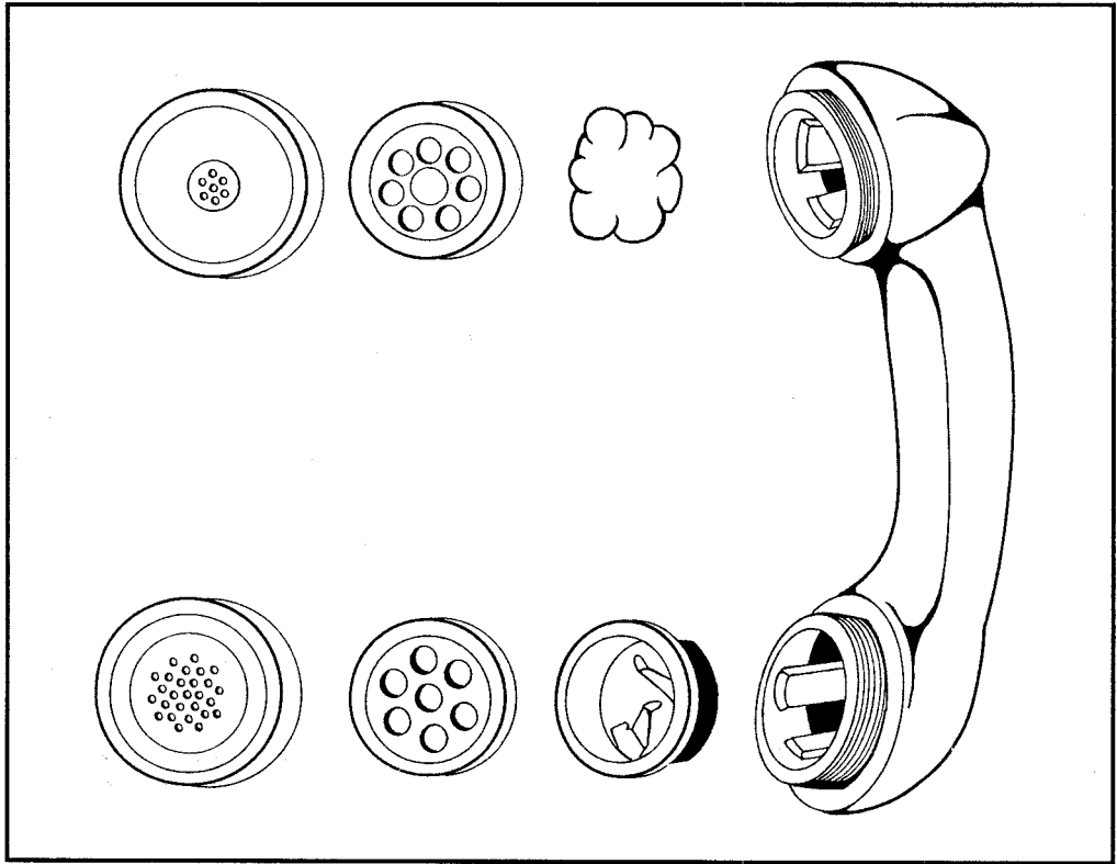
Figure 3: Exploded view of a standard handset
