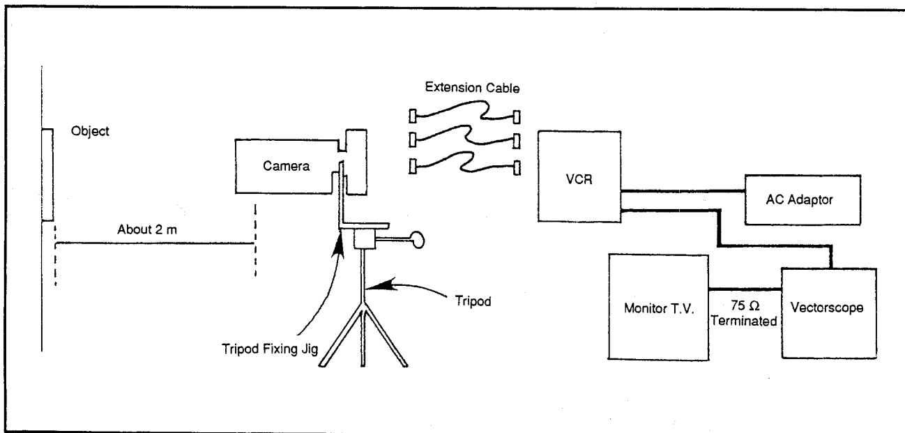
Figure 11: Set up for testing and adjusting
