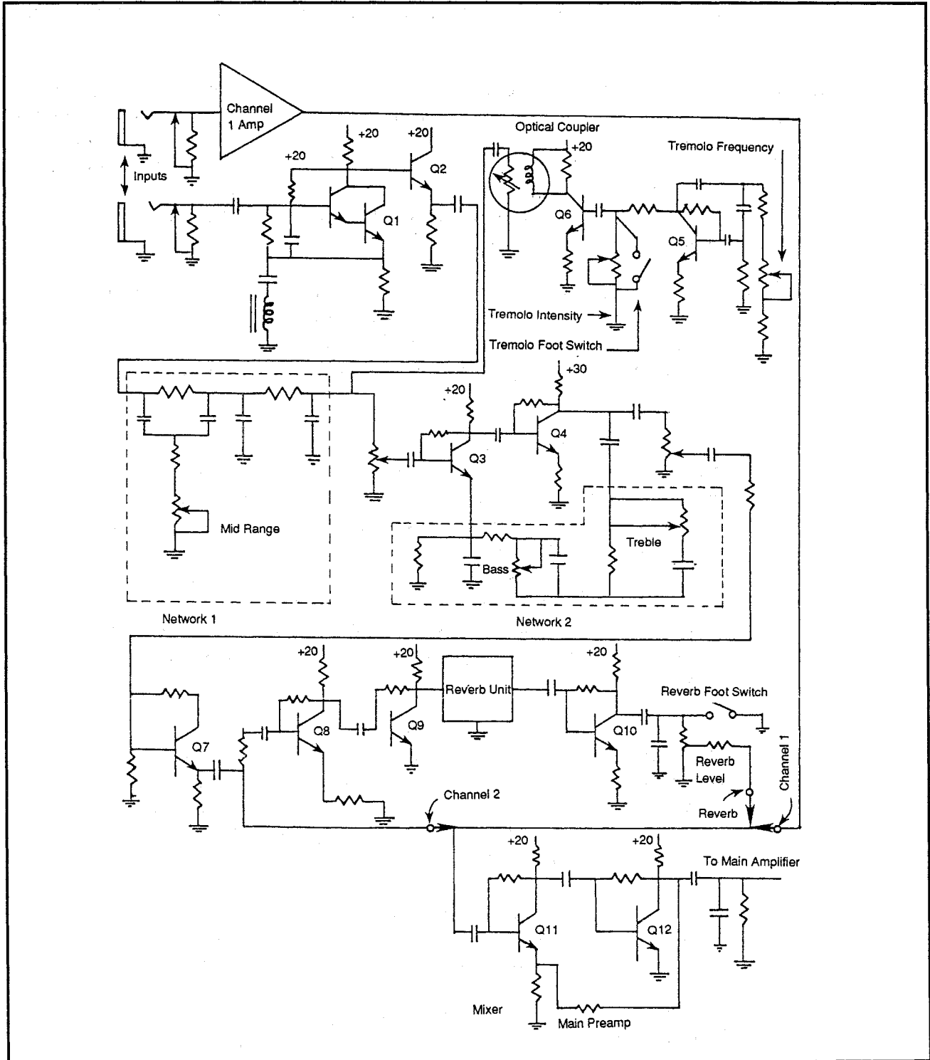
Figure 2: Solid-state preamplifier
