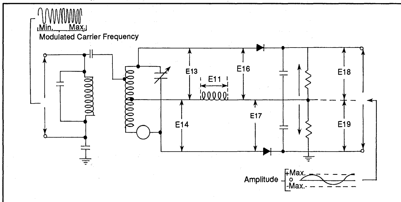
Figure 4: Discriminator circuit
