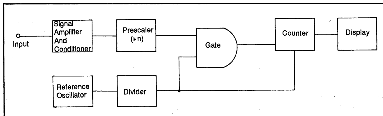
Figure 9: A prescaler circuit
