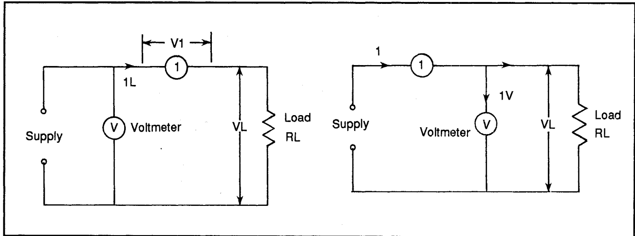
Figure 5: Current testing circuit
