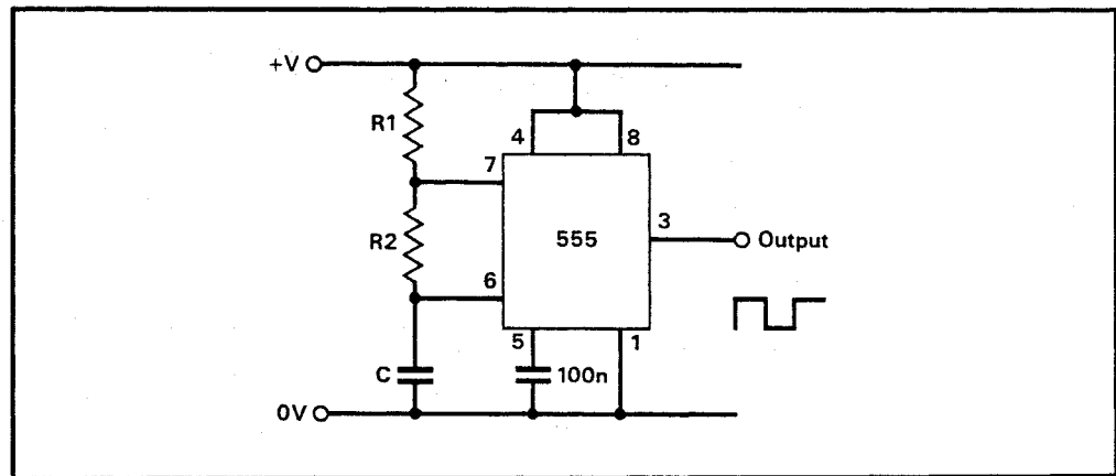
Figure 4: Astable pulse generator based on a timer
