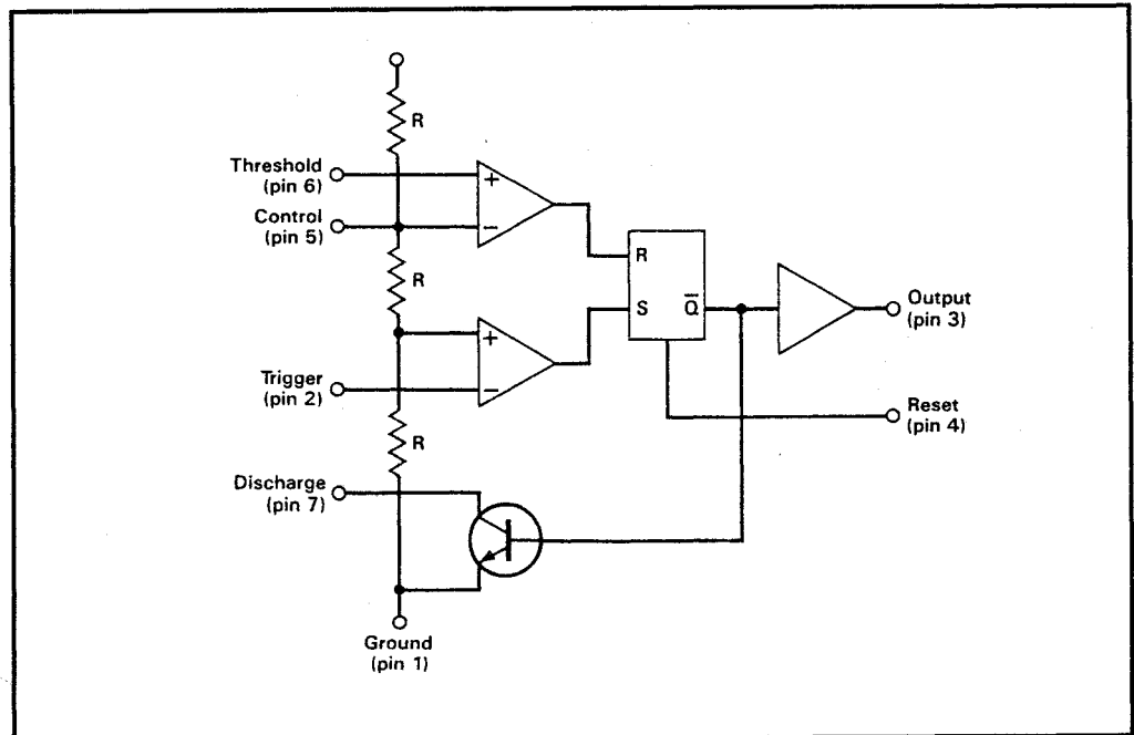
Figure 1: 555 timer
