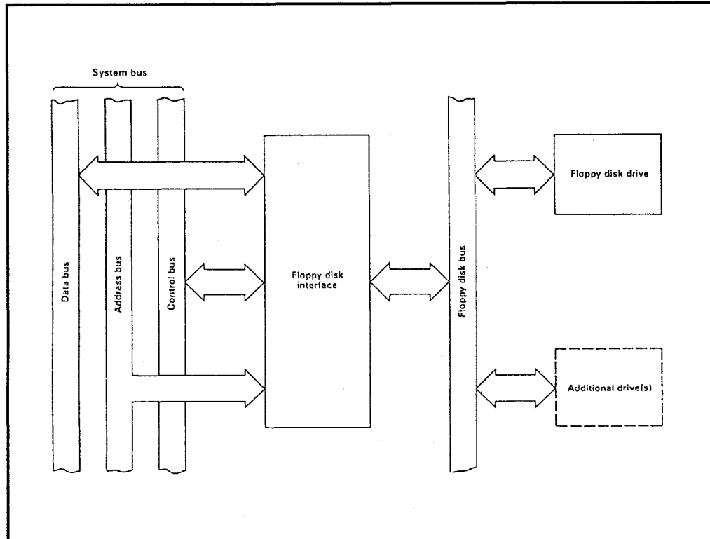
Figure 7: Floppy drive connector
