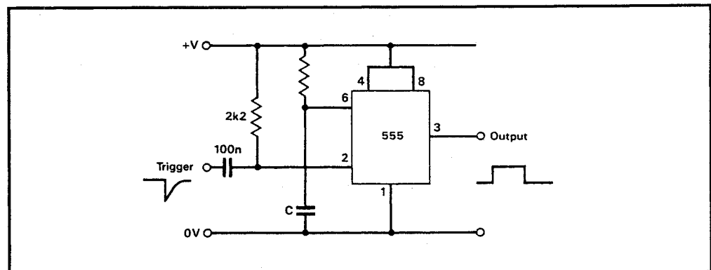
Figure 5: Monostable pulse generator based on a timer
