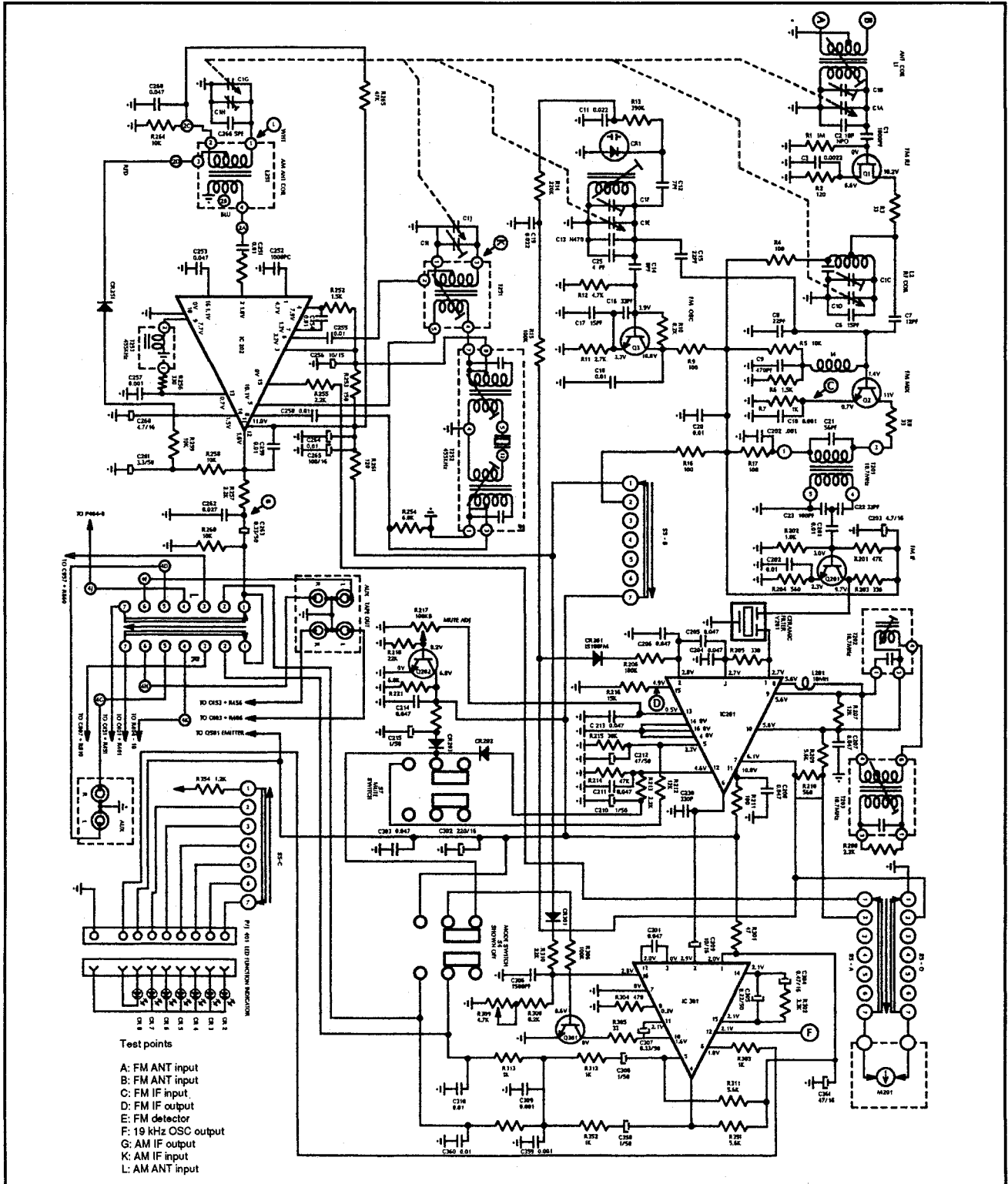
Figure 3: RF/IF/MPX schematic
