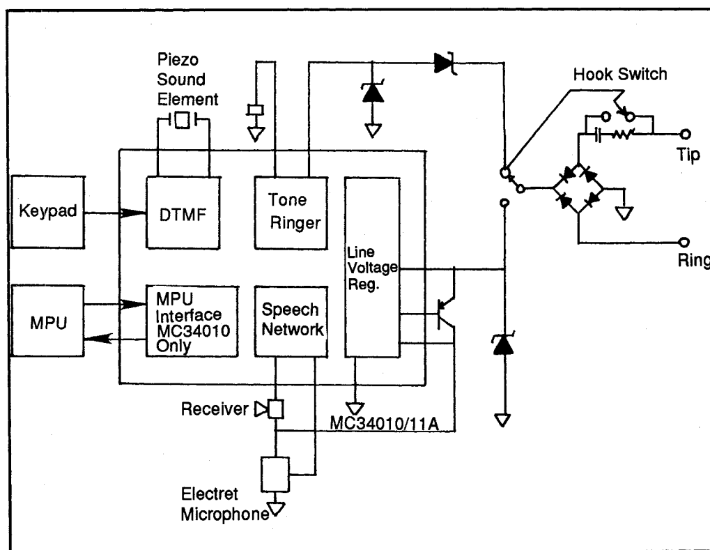
Figure 6: The complete, simplified electronic telephone
