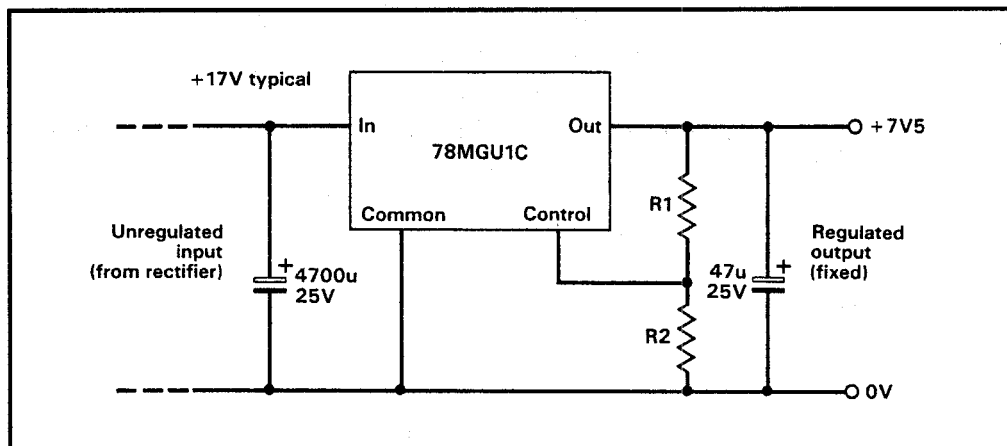
Figure 4: Variable voltage regulator with fixed output voltage
