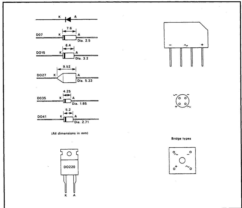
Figure 5: Diode casings
