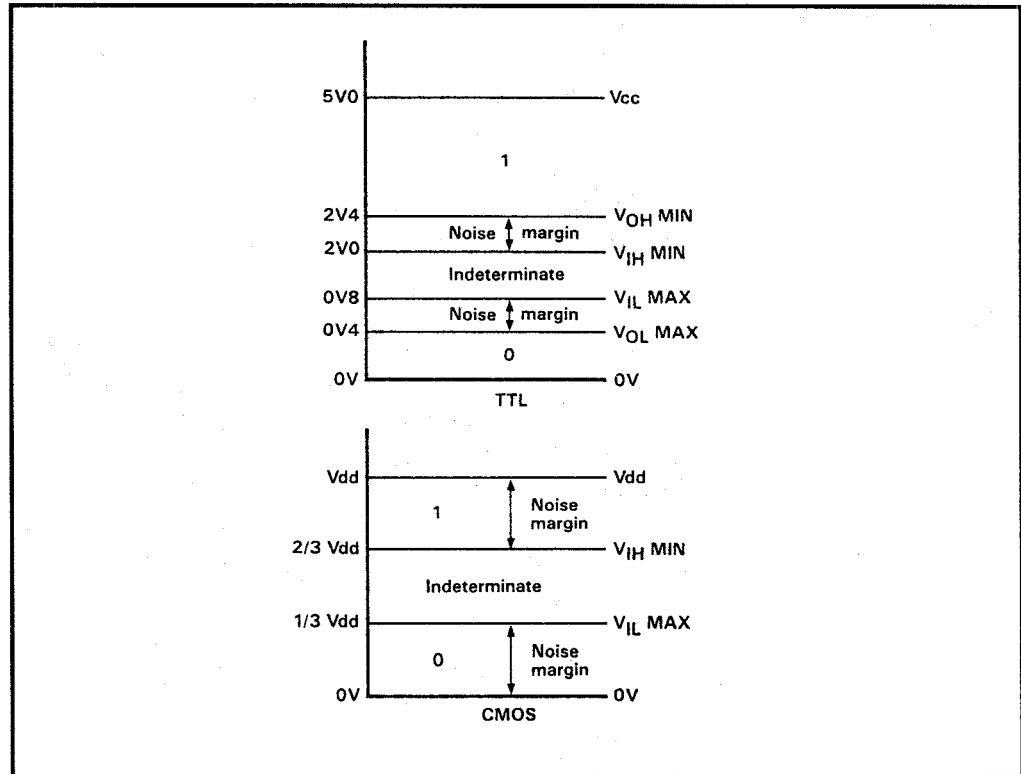
Figure 11: Logic levels and noise margins for CMOS and TTL Devices
