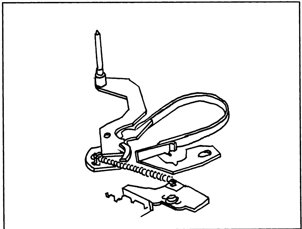
Figure 1: Back tension spring
