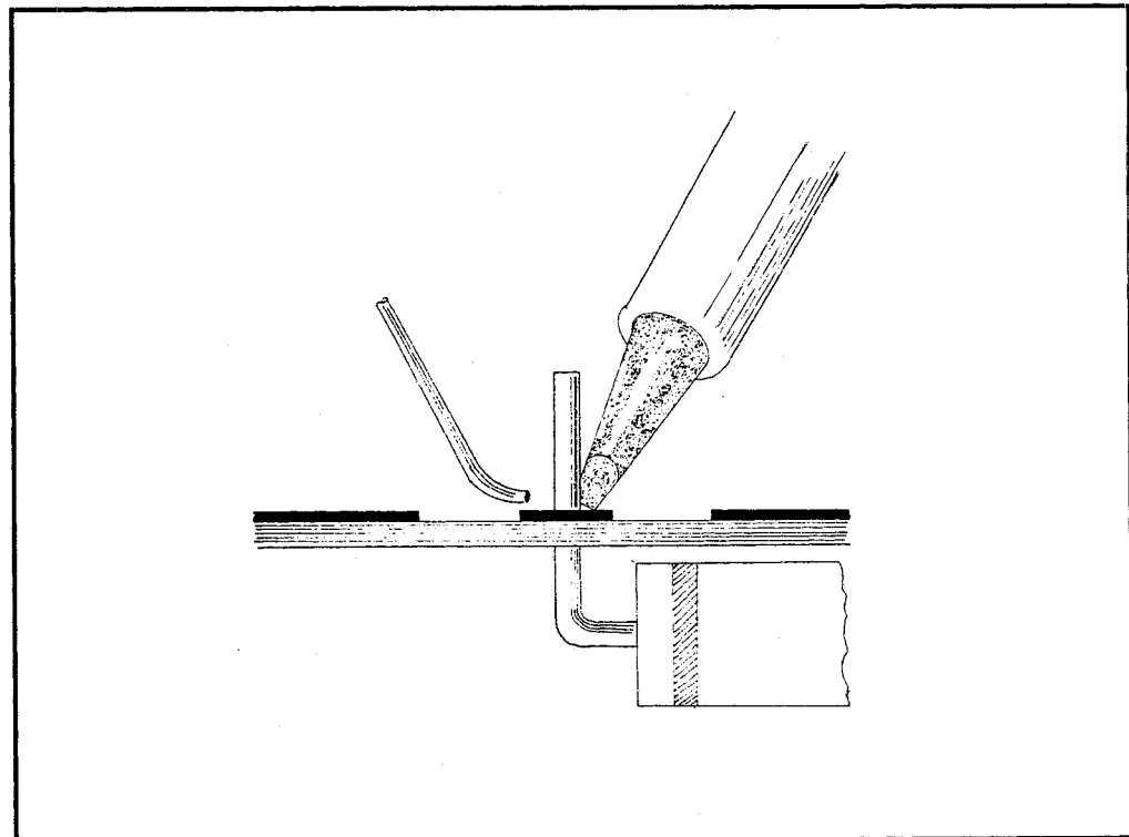
Figure 3: The soldering iron should heat the joint, with the joint melting the solder, not the soldering bit.
