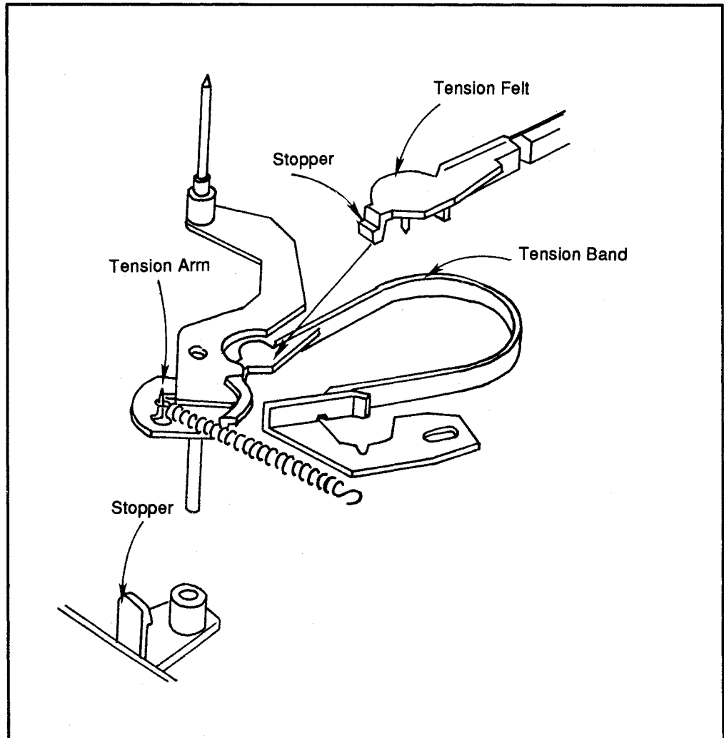
Figure 44: Tension band and tension arm assembly
