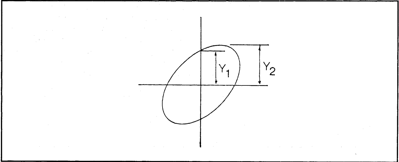
Figure 11: Measuring phase difference
