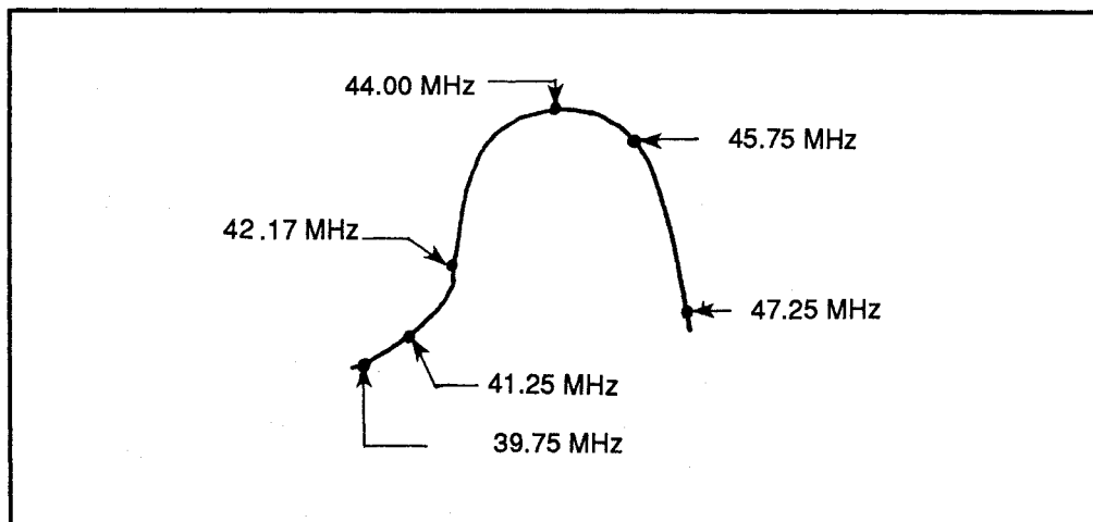
Figure 3: Waveform for adjustments from 39.75 MHz to 47.25 MHz
