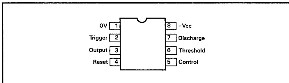
Figure 2: 555 timer pin connections
