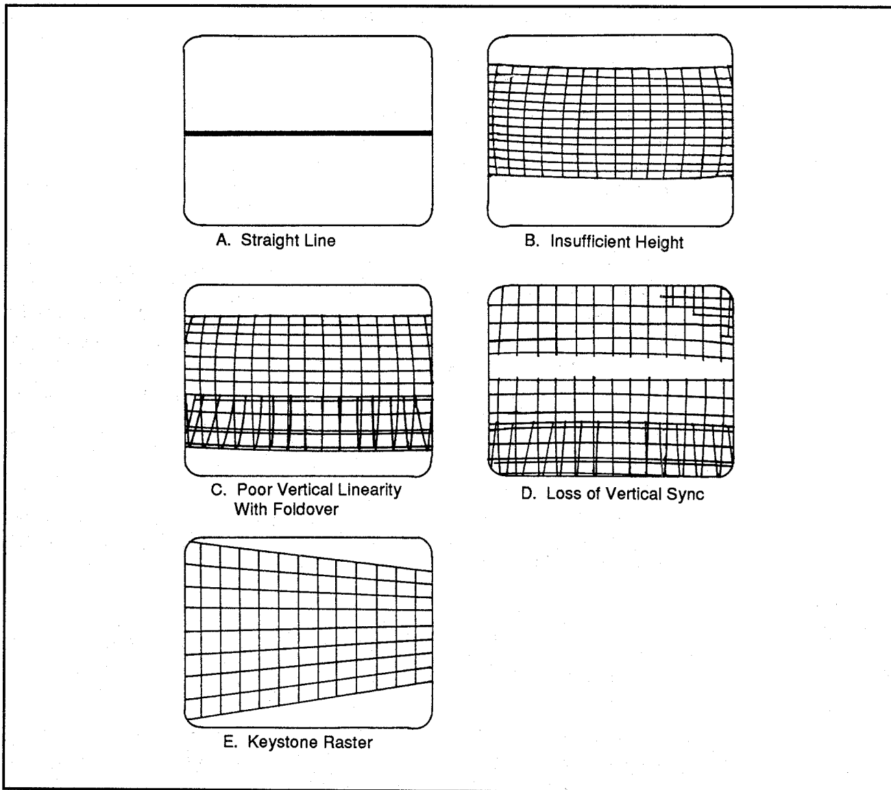
Figure 2: Video problems caused by vertical deflection malfunction: (a) loss of vertical deflection (b) improper height (c) improper vertical linearity (d) loss of vertical sync (d) keystoneing
