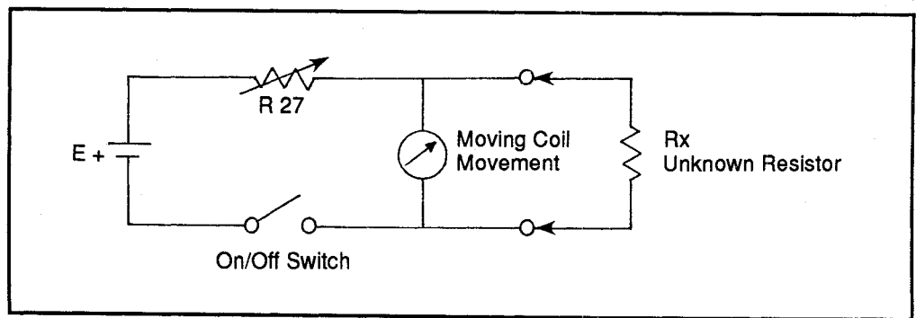
Figure 6: Resistance checking circuit
