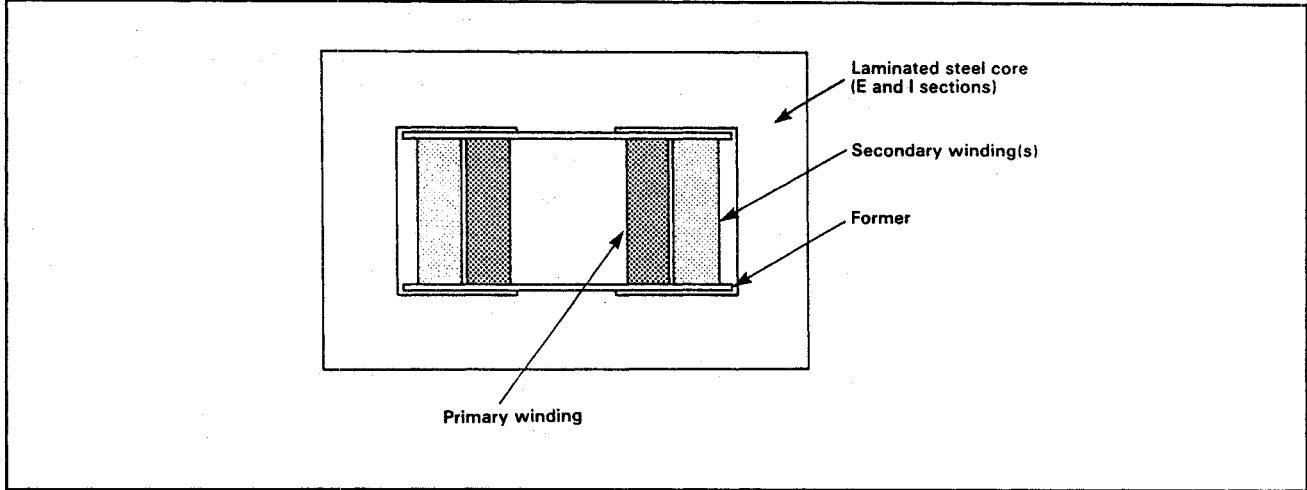
Figure 2: Transformer construction
