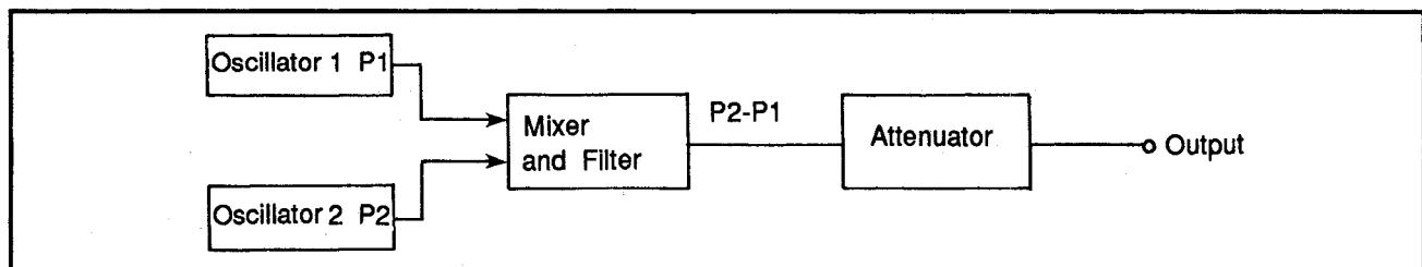
Figure 8: Heterodyne
