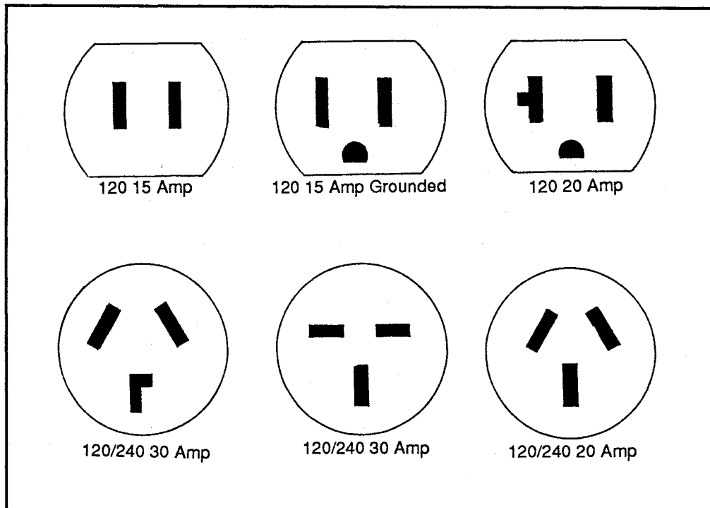
Figure 1: Receptacle types
