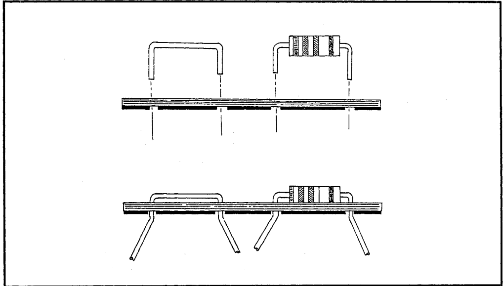
Figure 2: Fitting the components in the PC board holes, and bending the leads to hold them in place.
