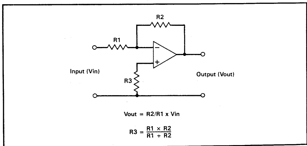
Figure 2: Operational amplifier with feedback
